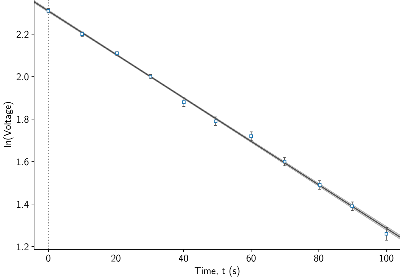
ln(Voltage) vs Time (Linear Fit)
