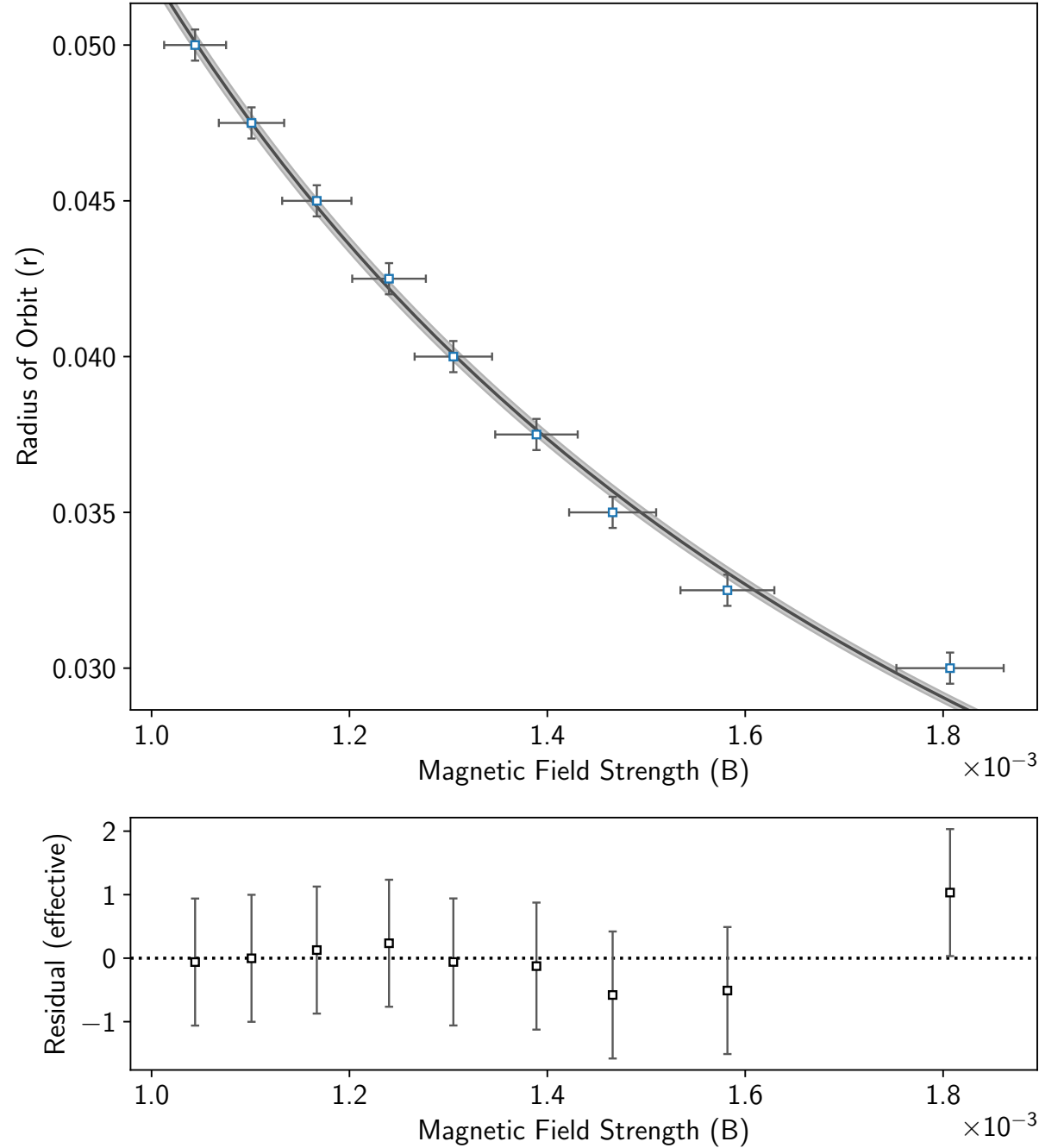
The Effect of Magnetic Field Strength on an Electron's Orbital Radius
