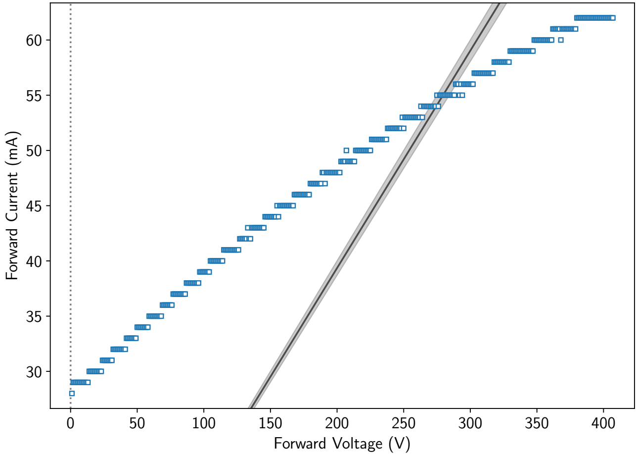
Cree Led RED XPEBRD-L1-0000-00901
