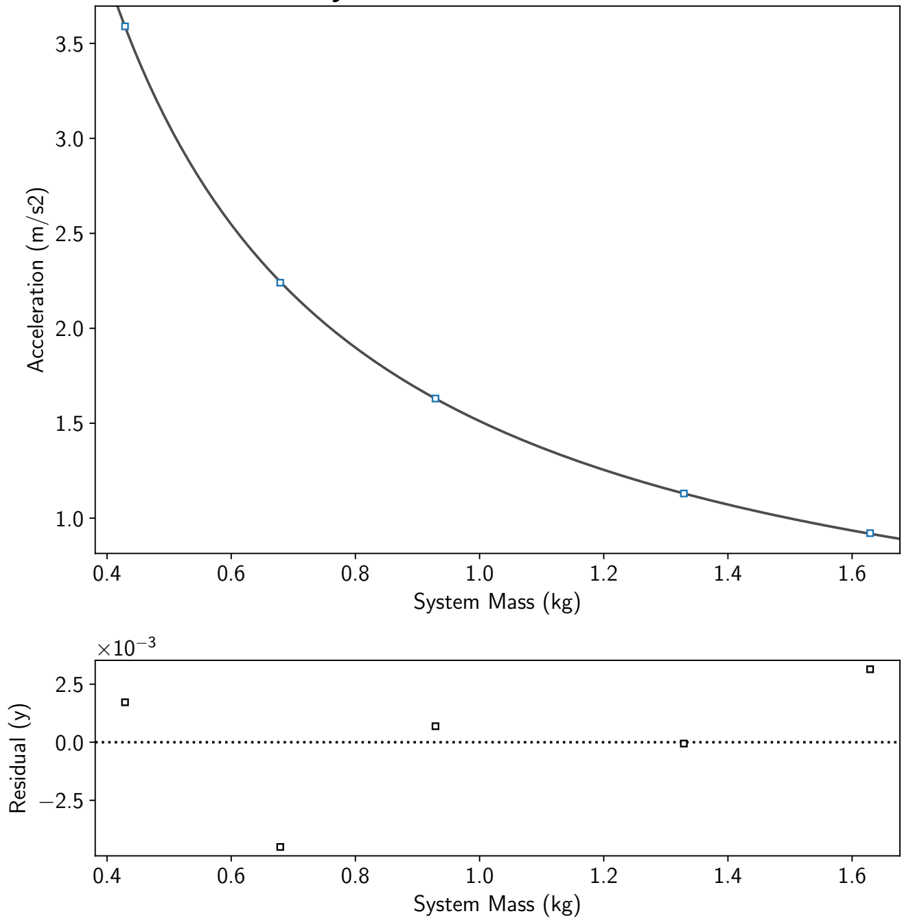
System Mass vs Acceleration
