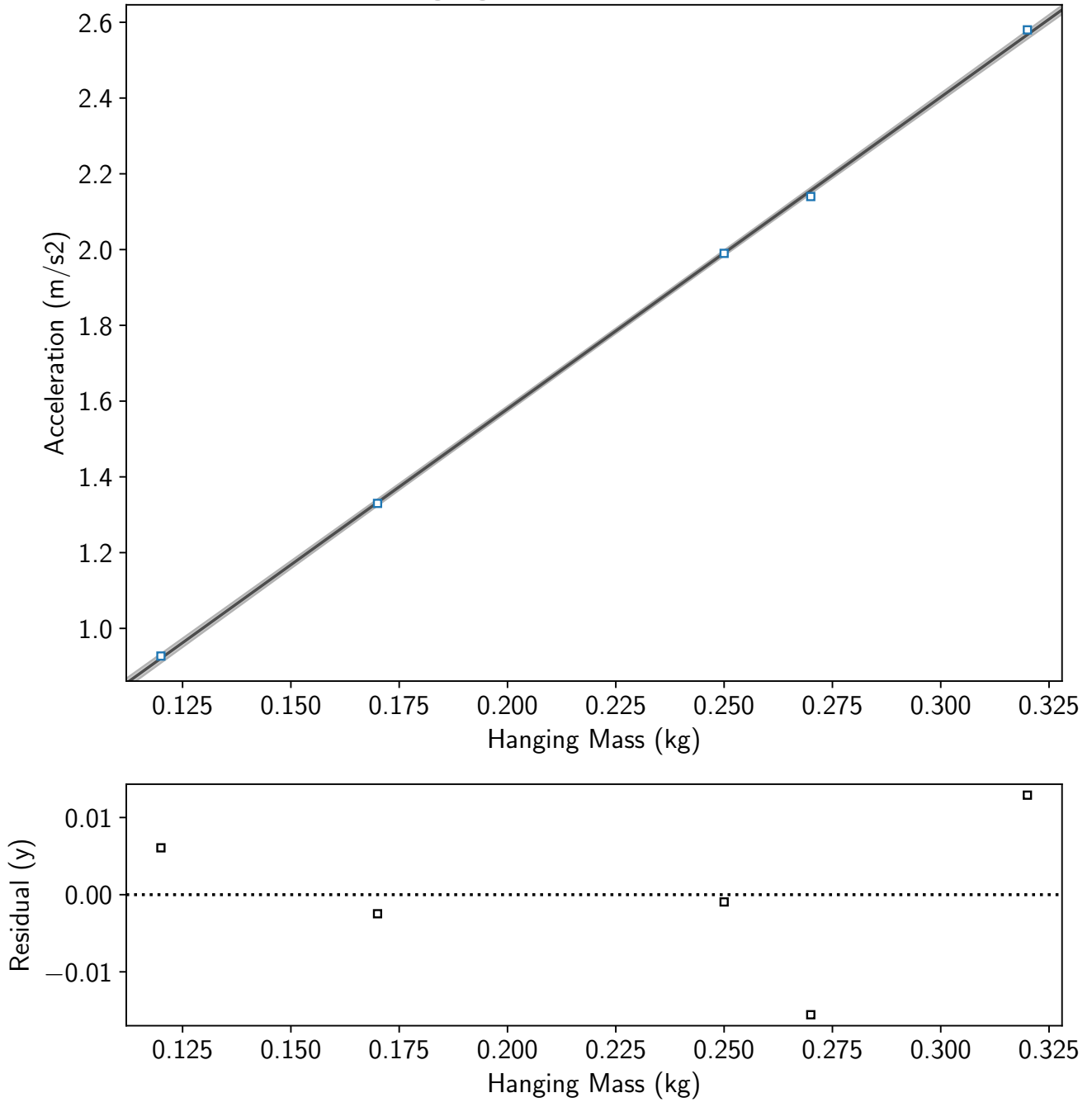
Hanging Mass vs Acceleration
