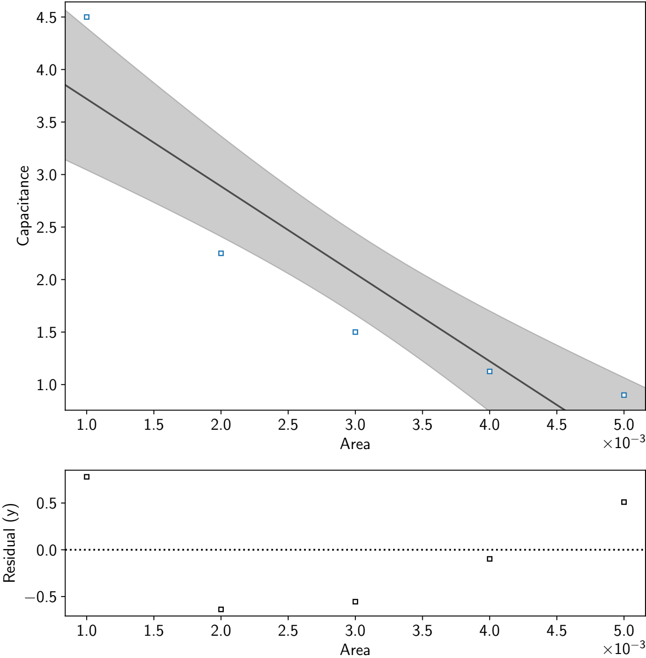
Capacitance vs. Area
