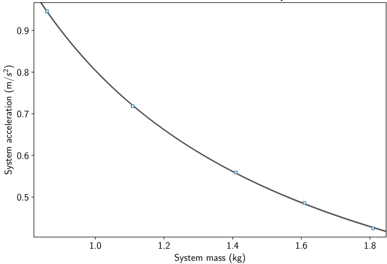
Fletcher Lab Power Law Graph
