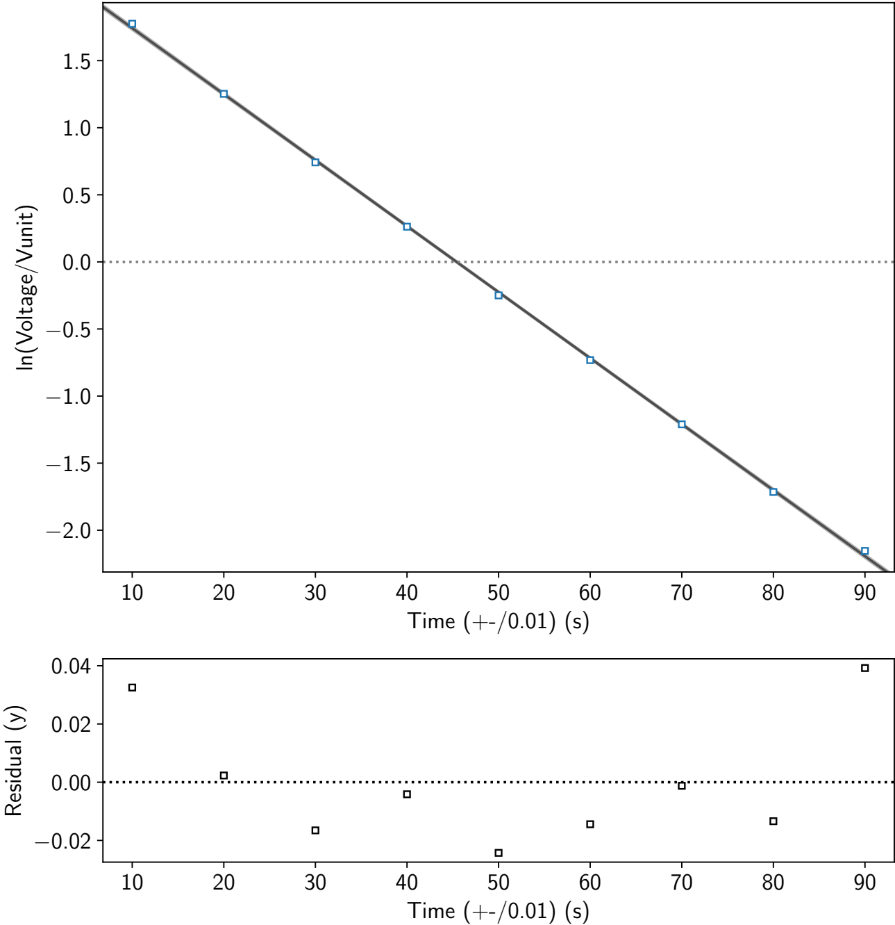
Discahring capacitors
