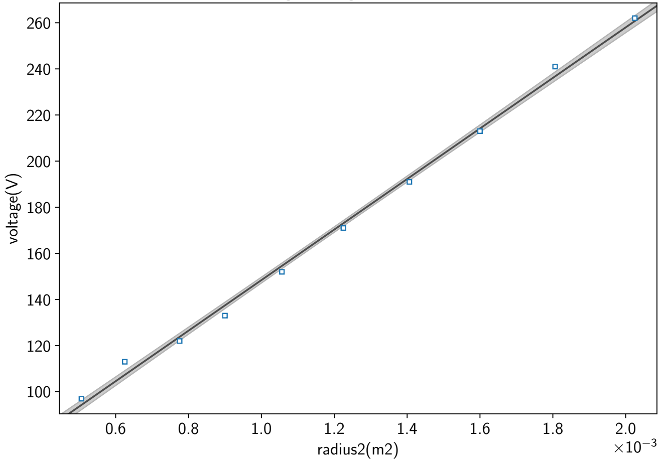
accelerating voltage vs radius squared
