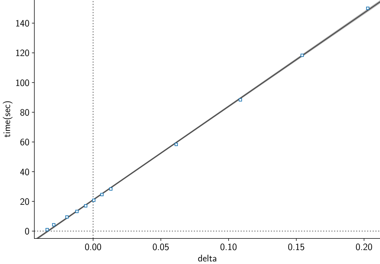
Capacitance time constant(liner) PT2
