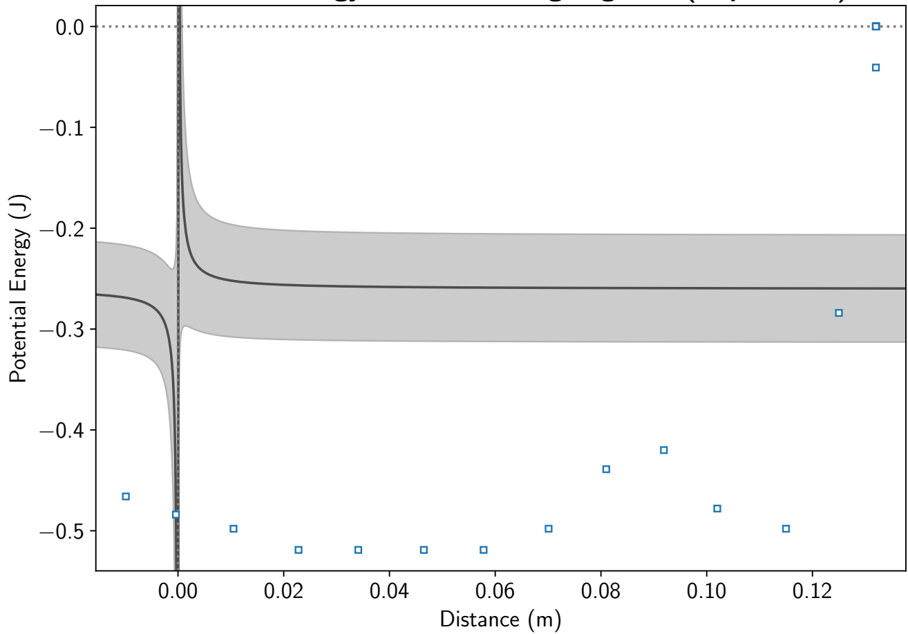
Potential Energy Curve for Outgoing Ball (Replicate 5)
