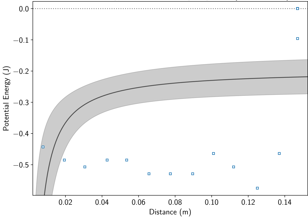
Potential Energy Curve for Outgoing Ball (Replicate 4)
