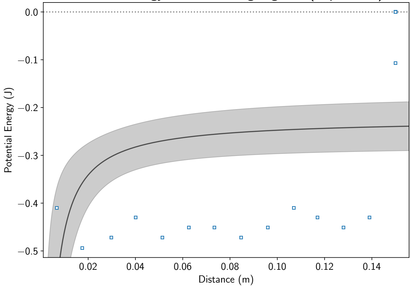
Potential Energy Curve for Outgoing Ball (Replicate 2)
