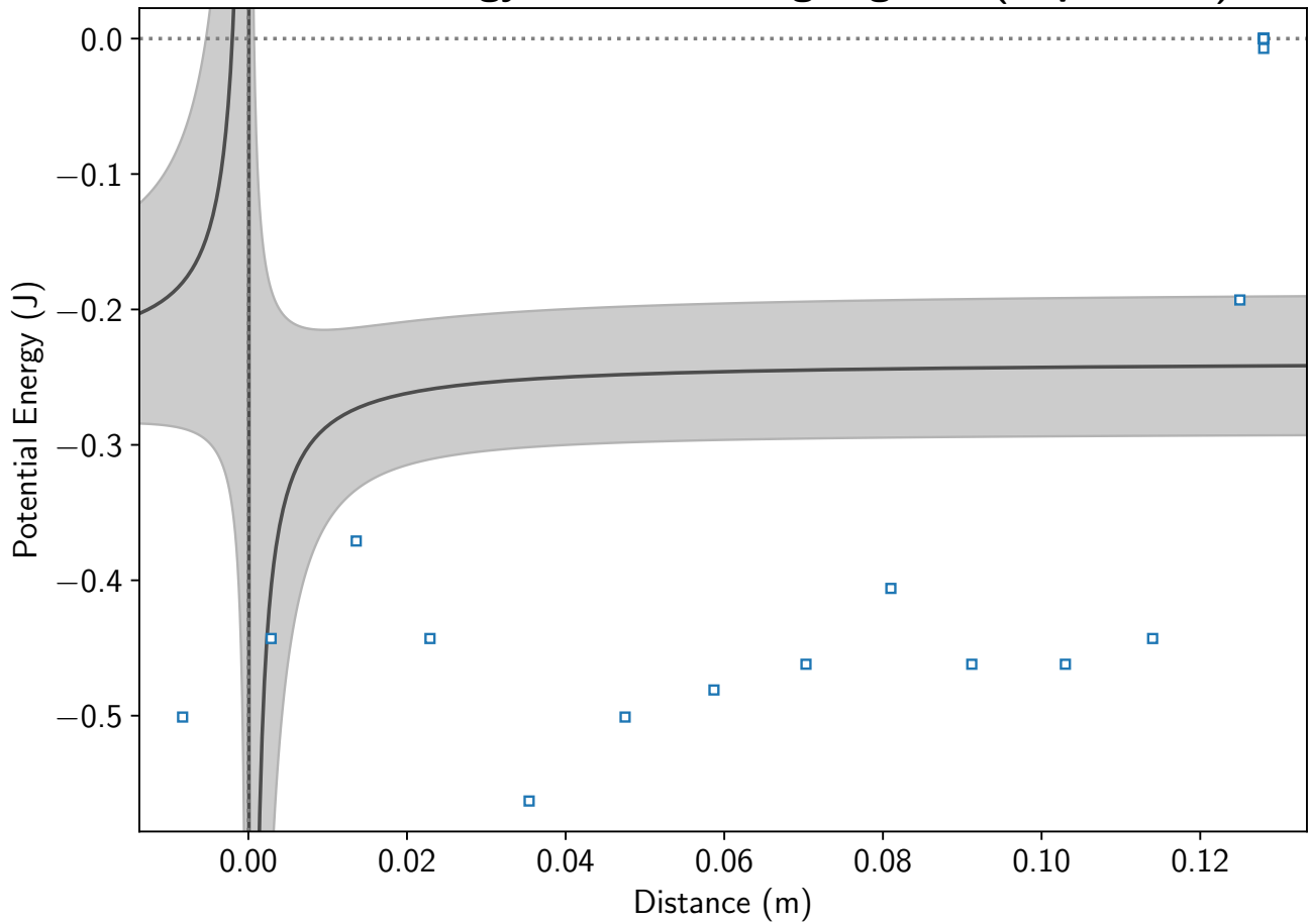
Potential Energy Curve for Outgoing Ball (Replicate 1)
