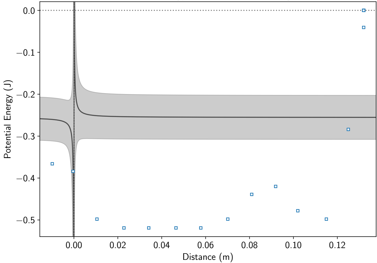
Potential Energy Curve for Incoming Ball
