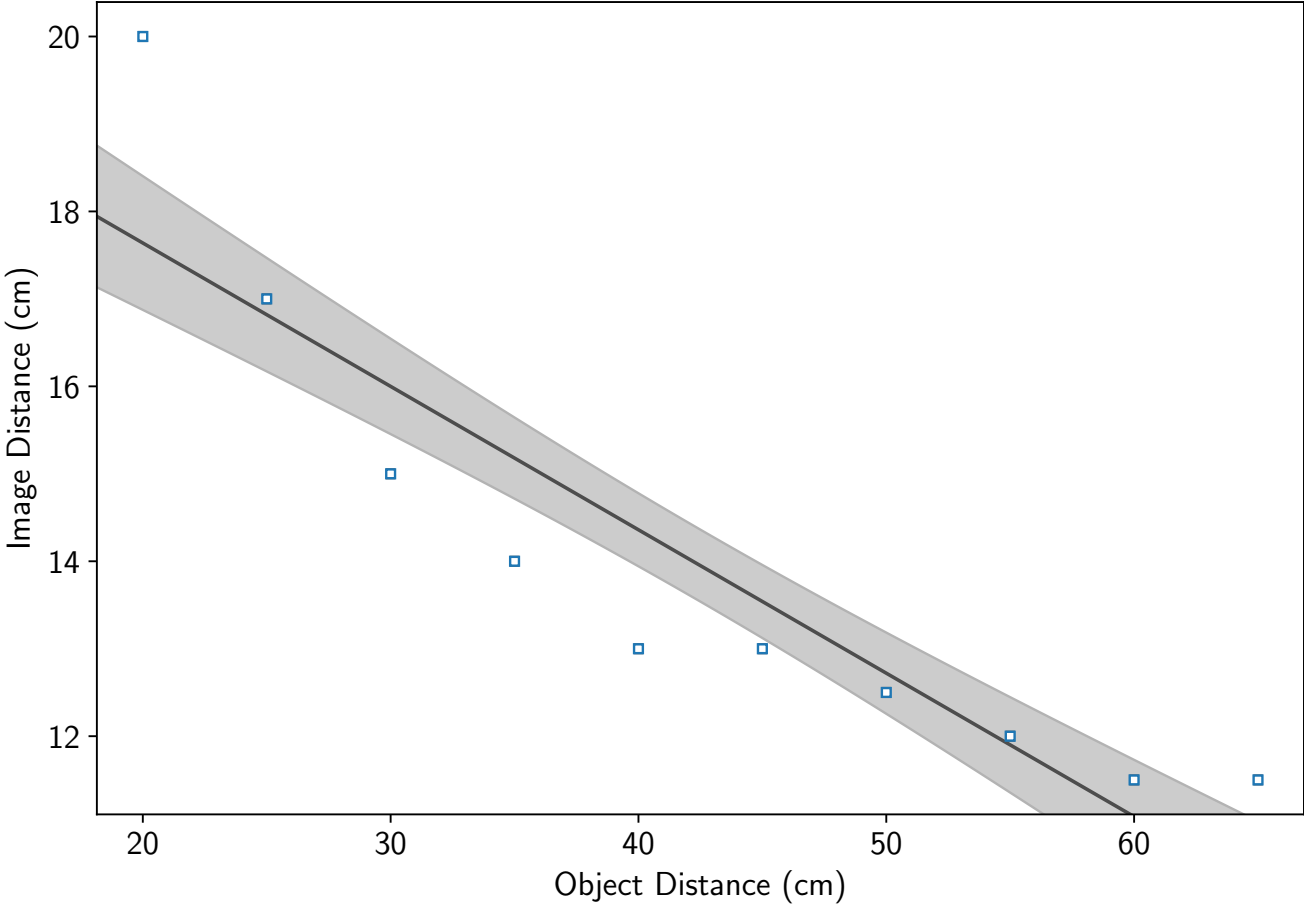
Object Distance (cm) vs. Image Distance (cm)
