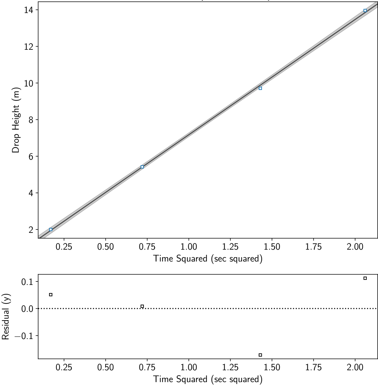
Ball Drop (stopwatch 3)
