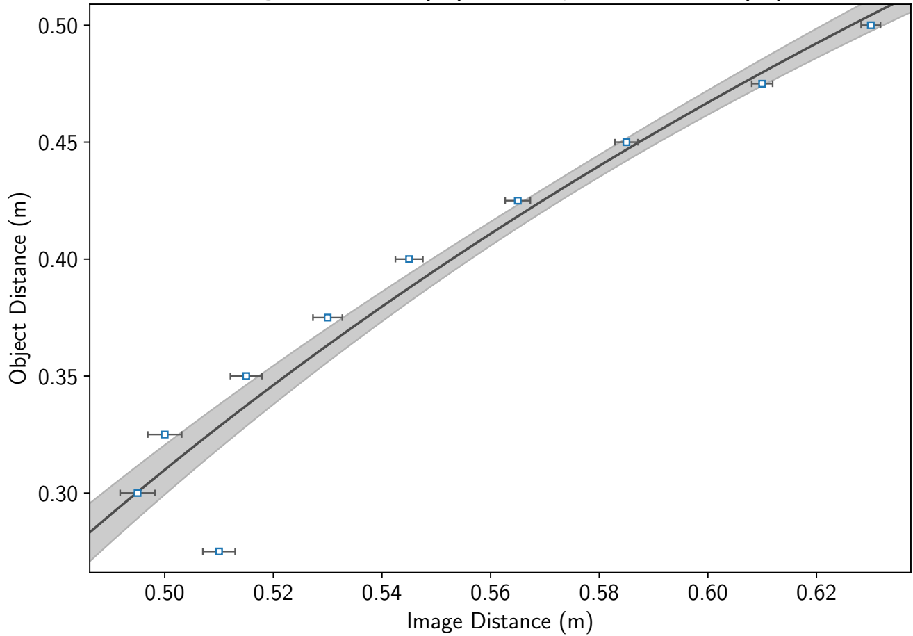
Image Distance (m) vs. Object Distance (m)
