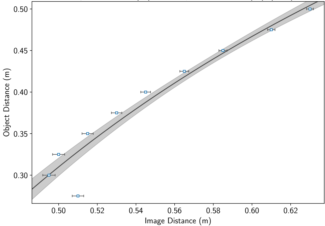
Image Distance (m) vs. Object Distance (m) (mm)
