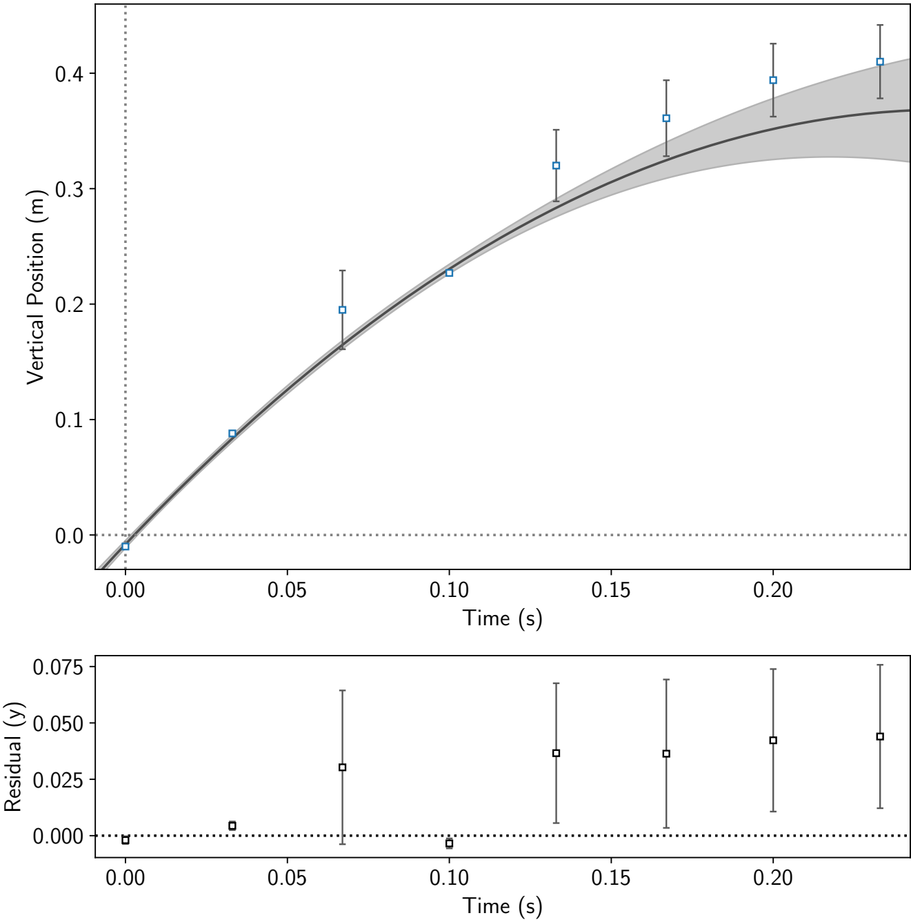
Vertical Upwards Throw of Mass 2 over time
