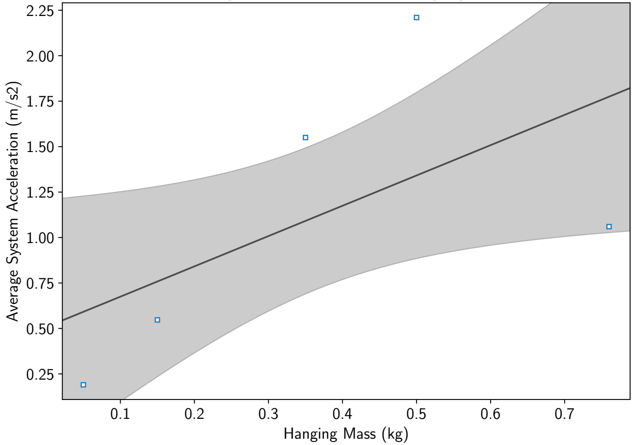
Average Acceleration vs Hanging Mass
