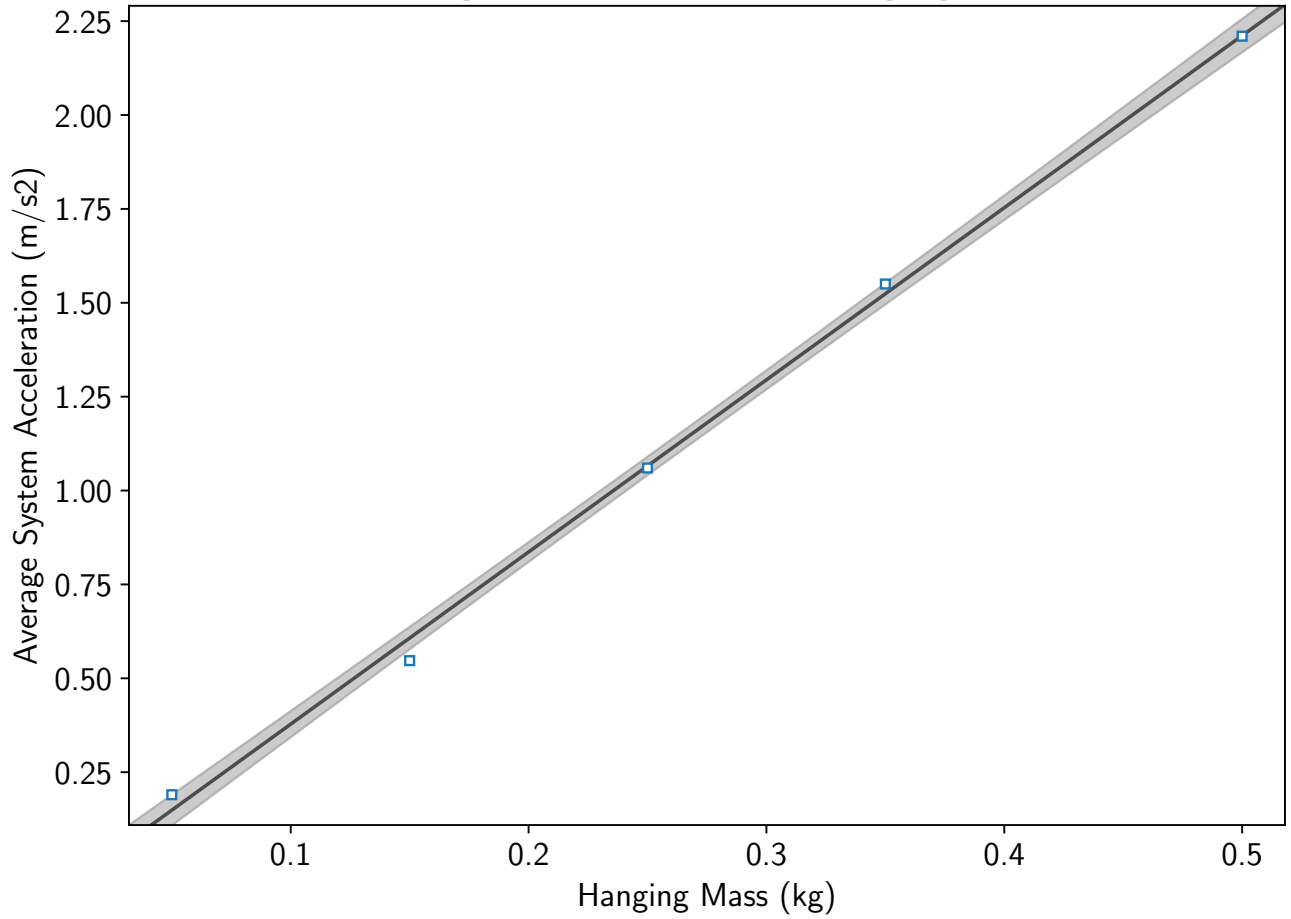
Average Acceleration vs Hanging Mass
