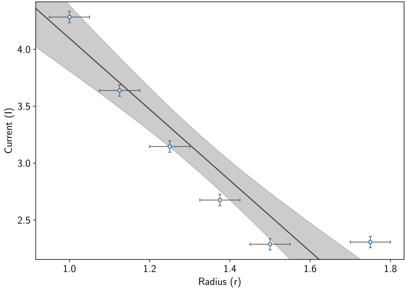
Relationship between Current and Radius for Va=150V
