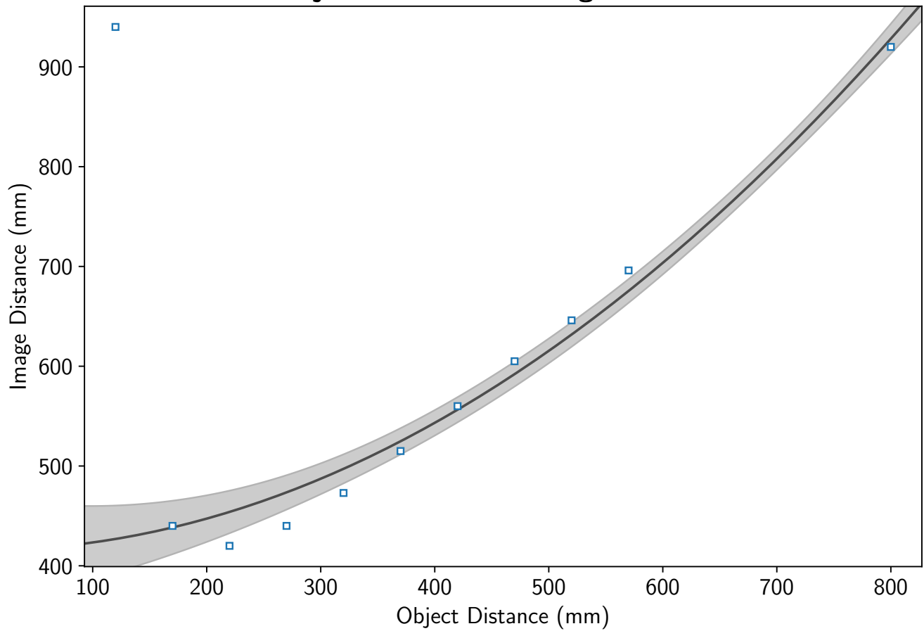
Object Distance vs Image Distance
