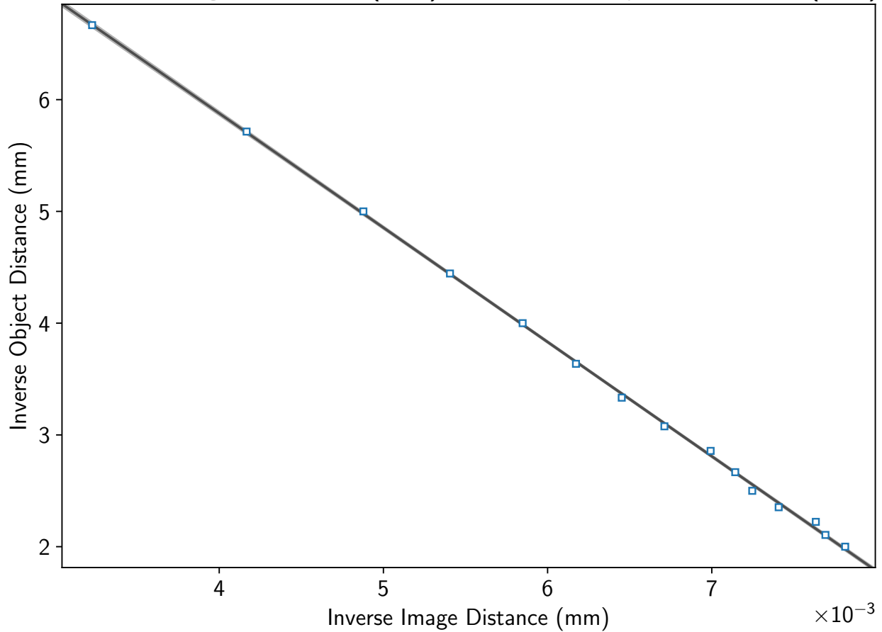
Inverse Image Distance (mm) vs Inverse Object Distance (mm)
