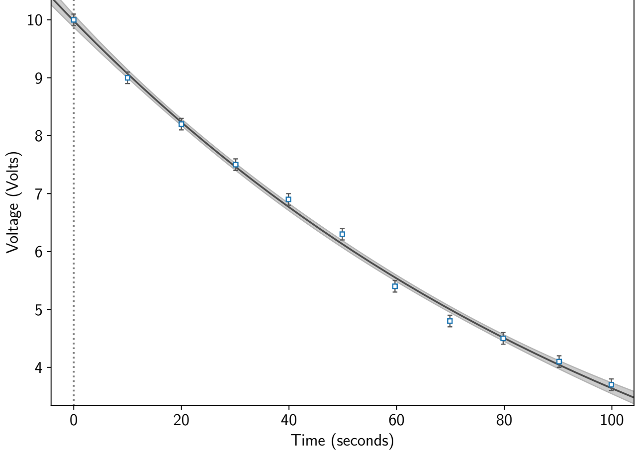
Voltage (V) VS. Time (s) (Semilog Fit)
