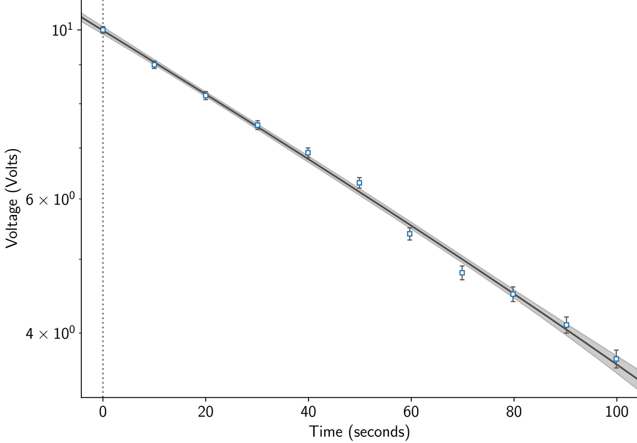
Voltage (V) VS. Time (s) (Semilog Fit)
