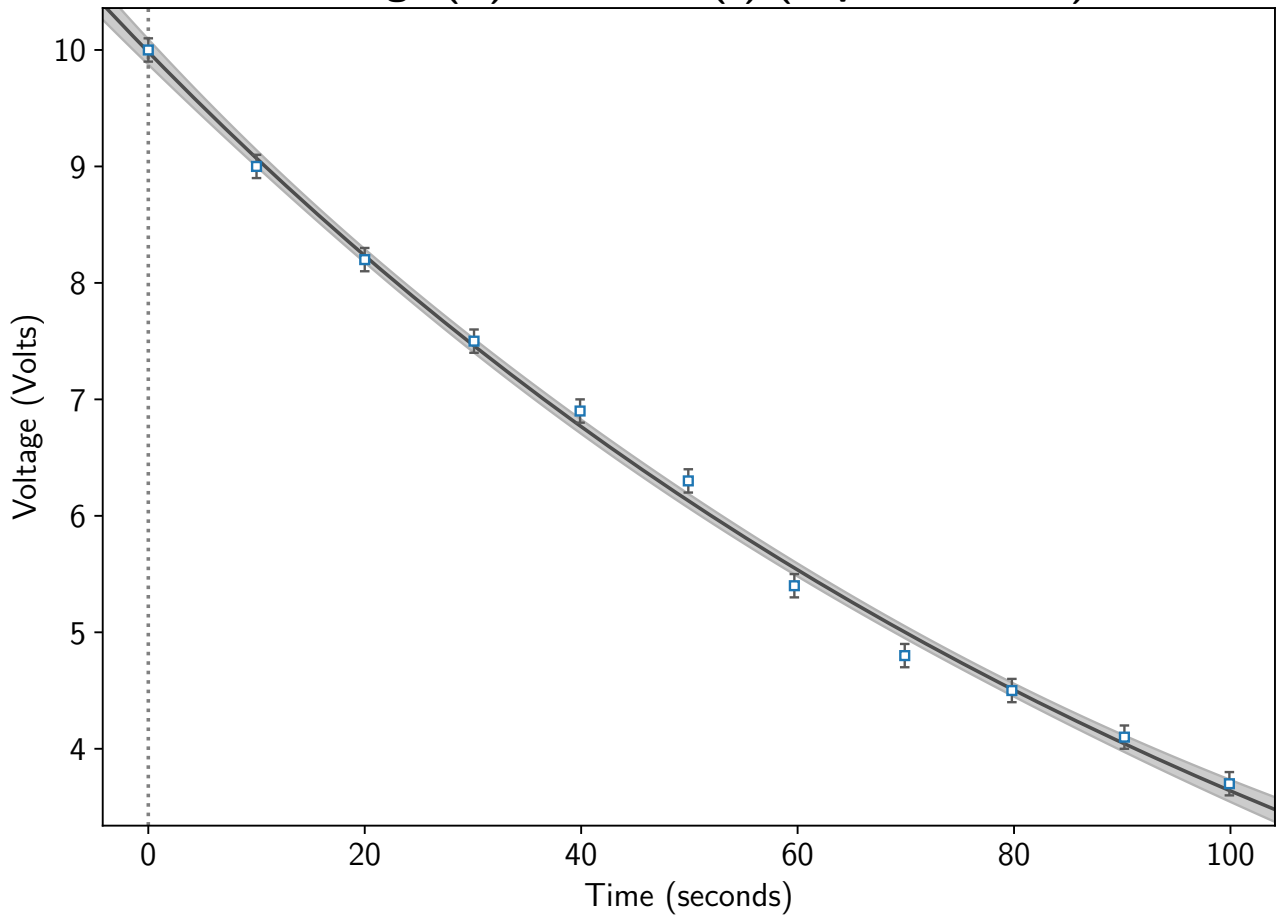
Voltage (V) VS. Time (s) (Exponential Fit)
