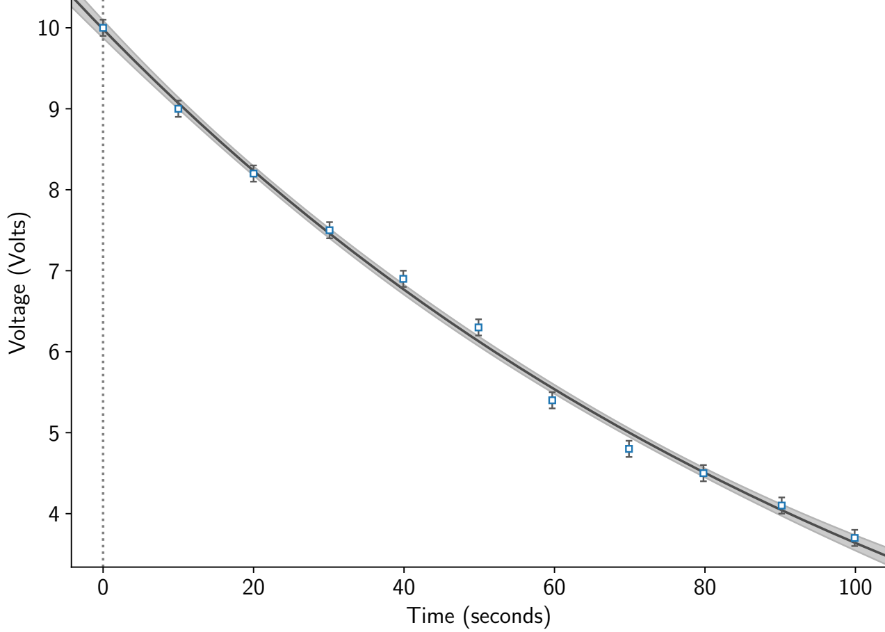
Voltage (V) VS. Time (s) (Converted Data)
