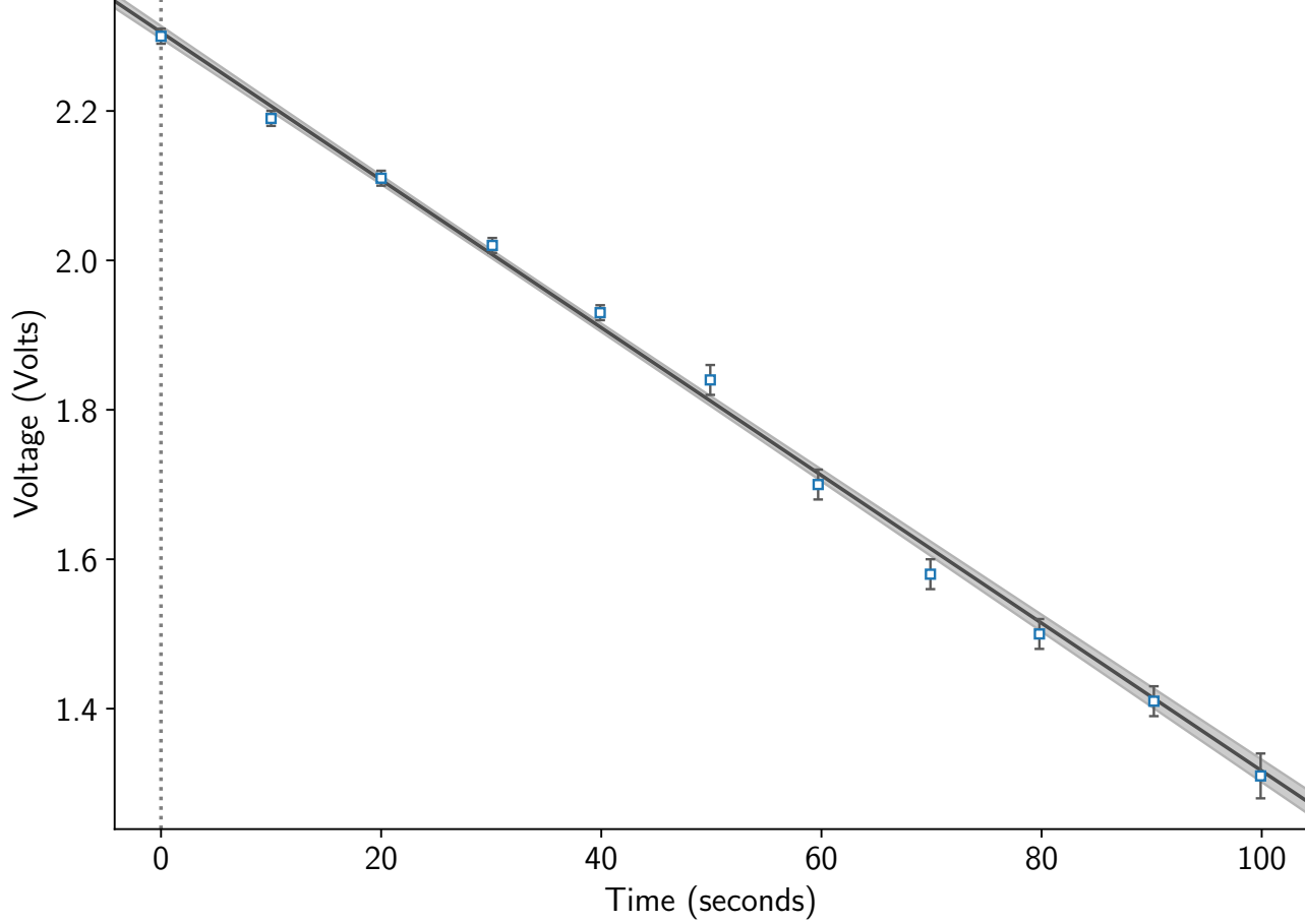
Voltage (V) VS. Time (s) (Converted Data)
