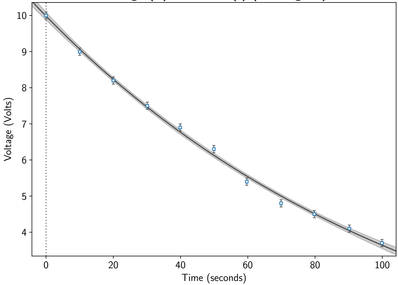
Voltage (V) VS. Time (s) (Semilog Fit)
