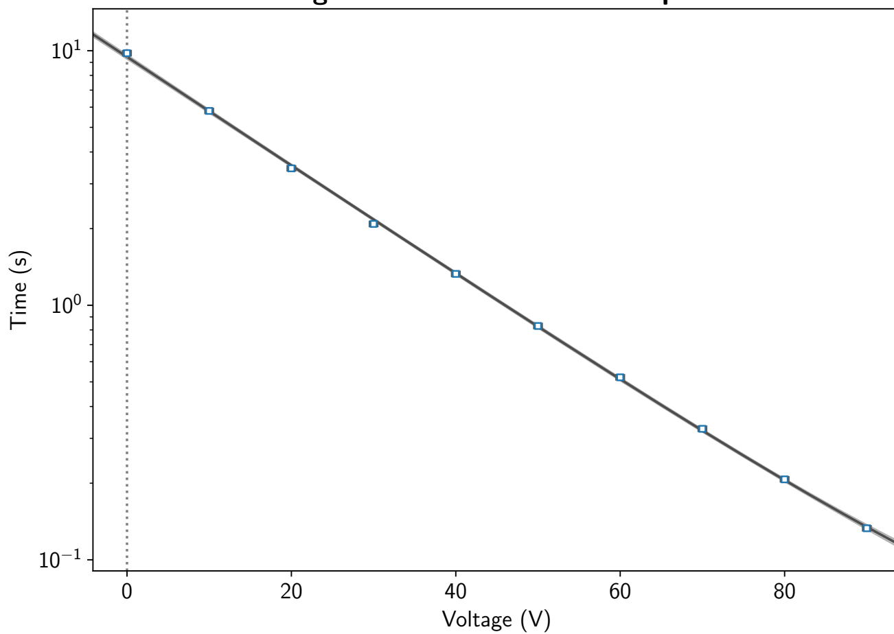
Voltage over Time of a 1.8UF capacitor
