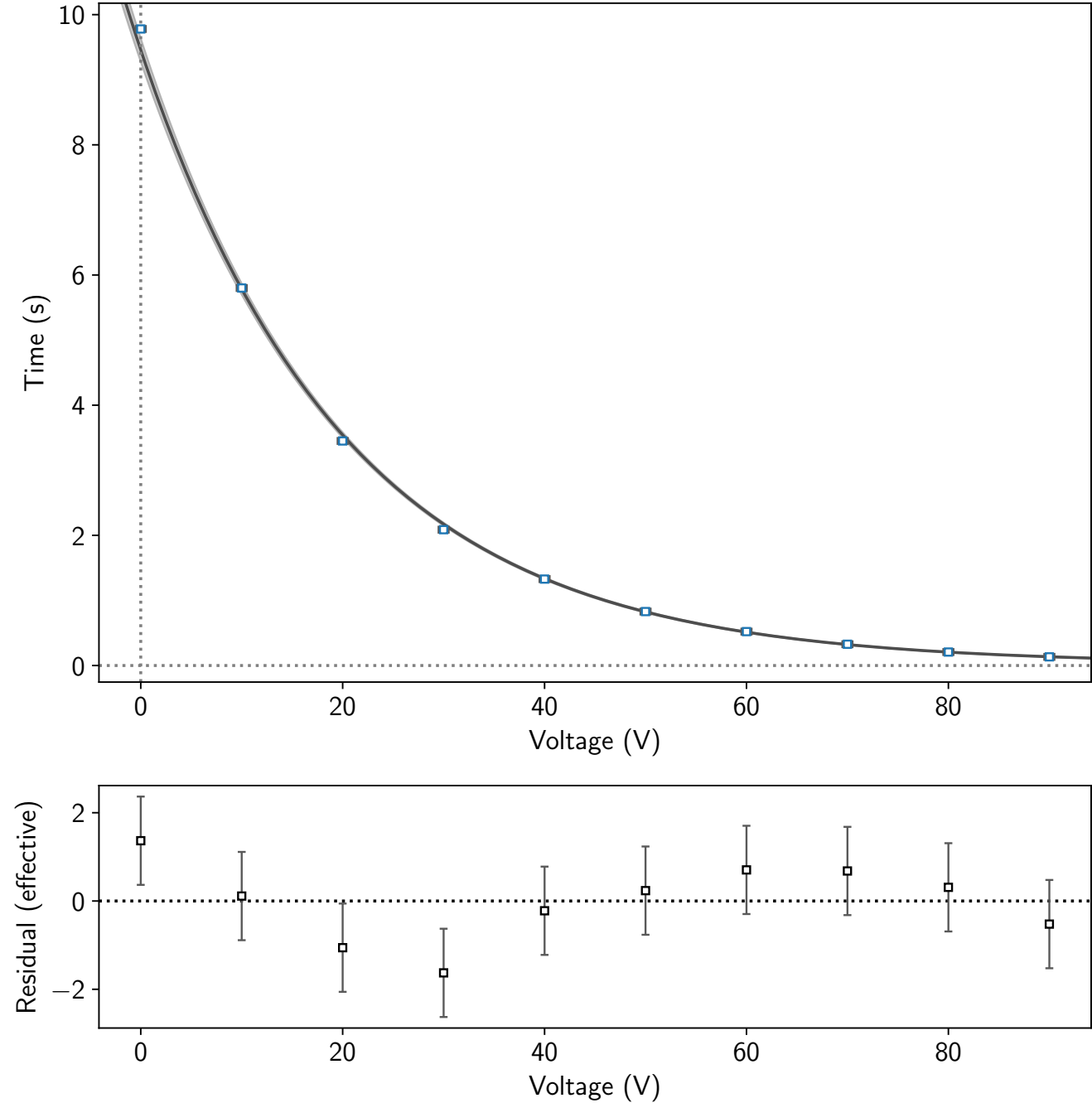
Time over Voltage of a 1.8UF capacitor
