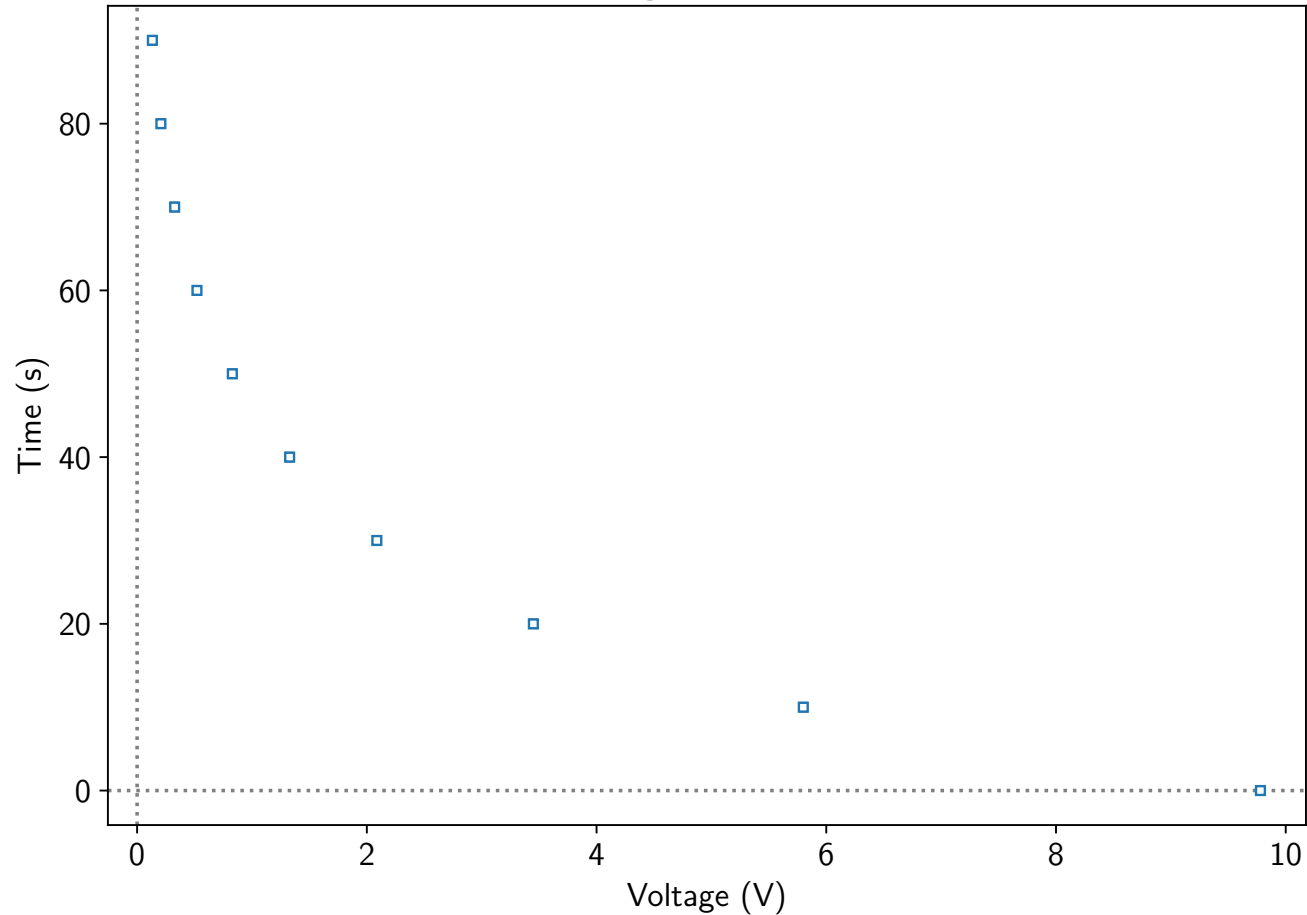
Time over Voltage of a 1.8UF capacitor
