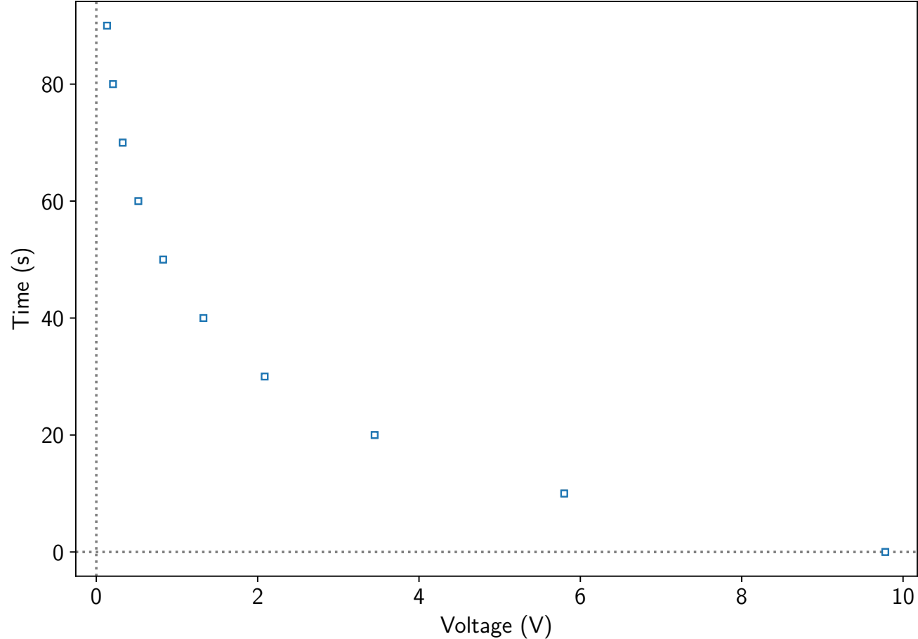
Time over ln(Voltage Unitless) of a 1.8UF capacitor
