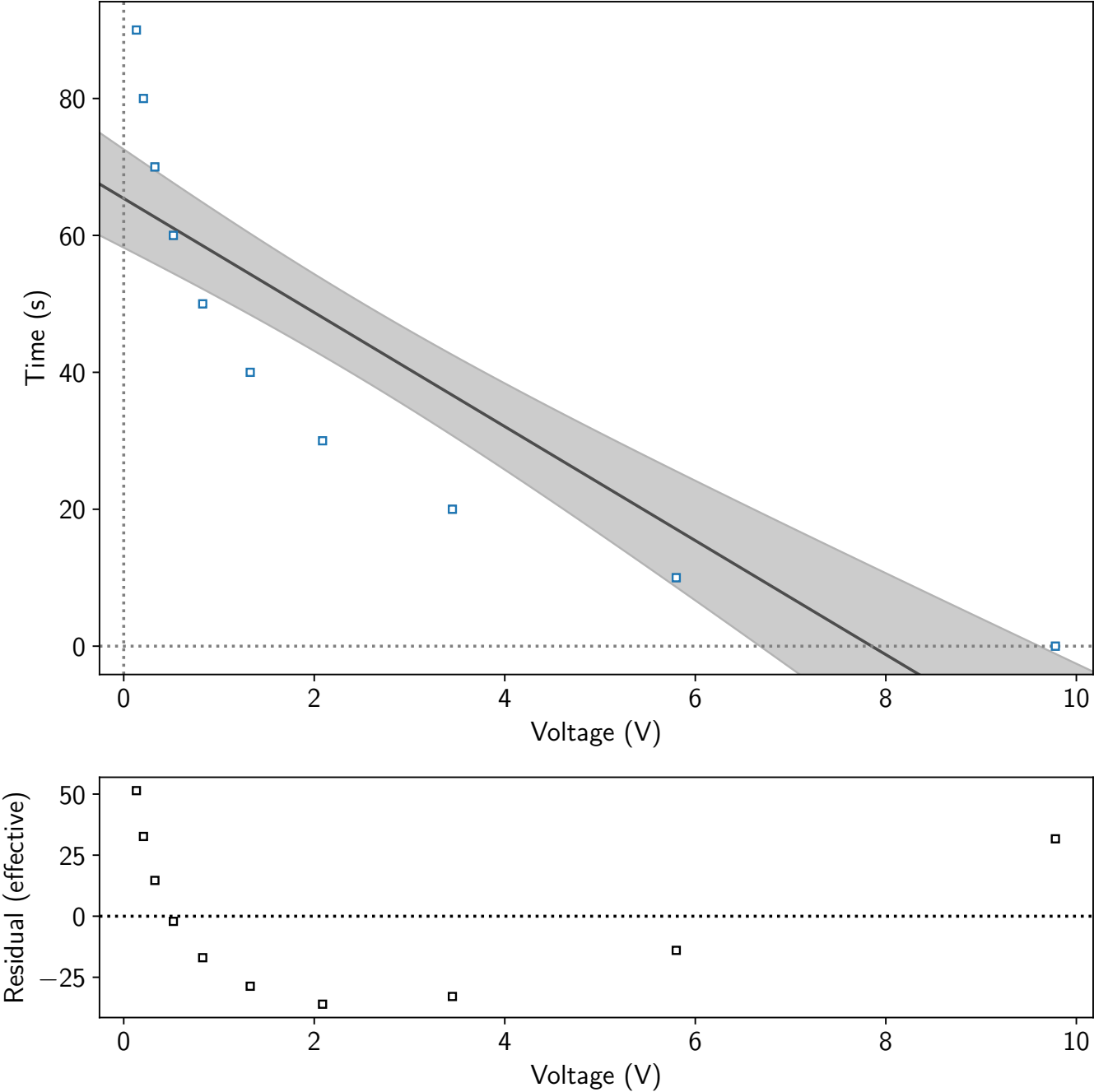
Time over ln(Voltage Unitless) of a 1.8UF capacitor
