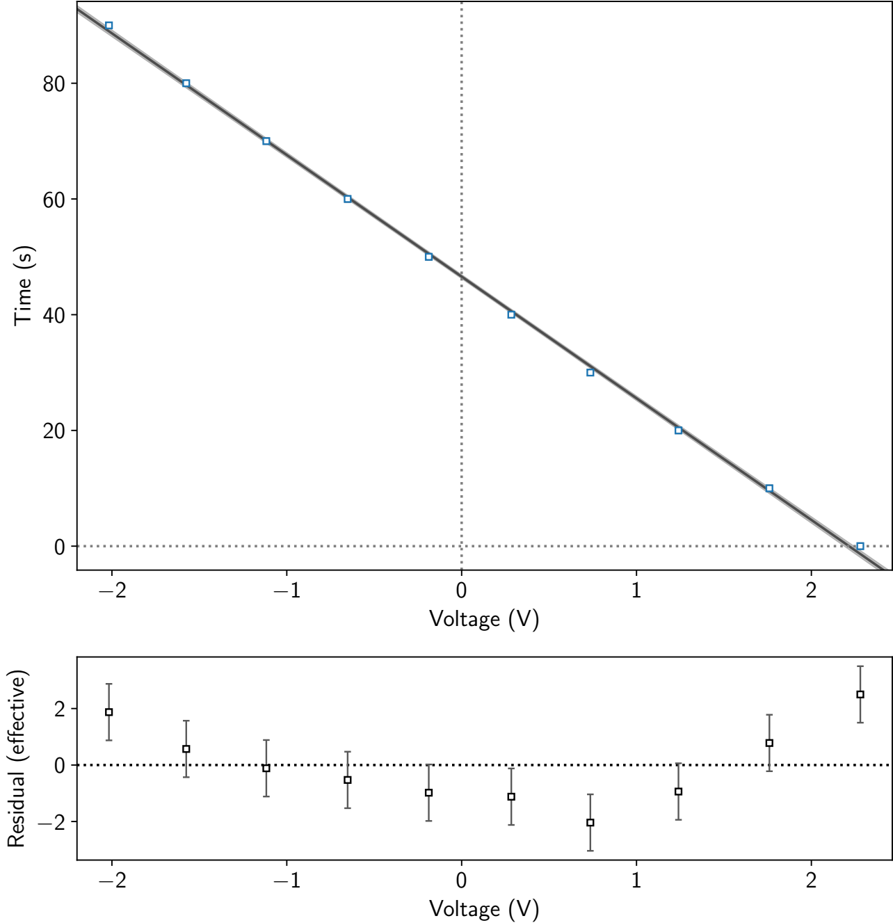
Time over ln(Voltage Unitless) of a 1.8UF capacitor
