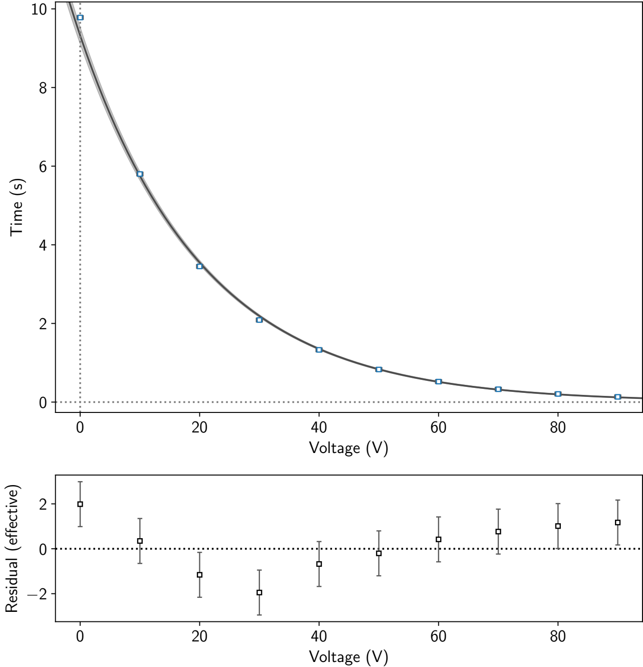
Time over Voltage of a 1.8UF capacitor
