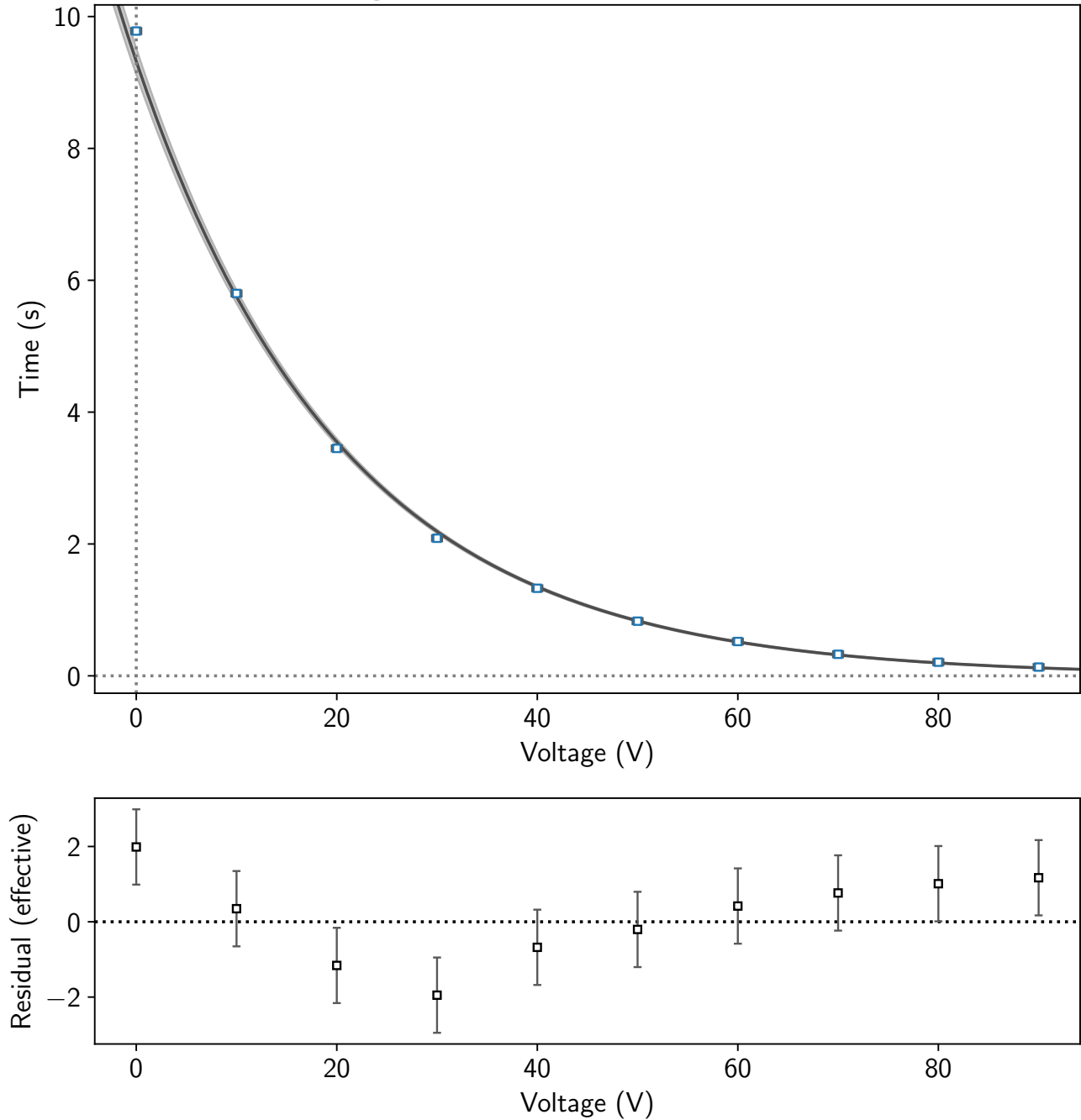
Voltage over time of a 1.8UF capacitor
