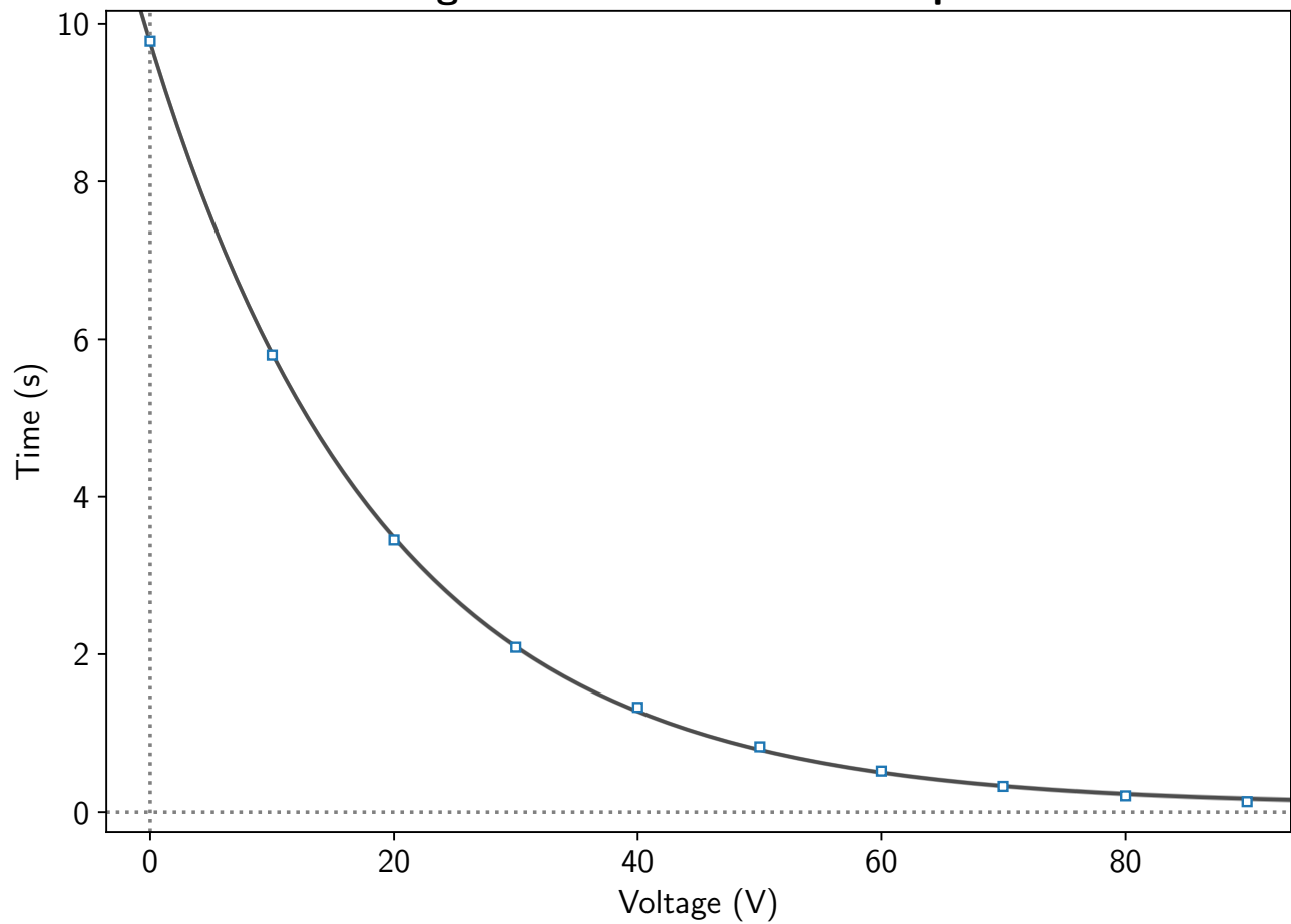
Voltage over time of a 1.8UF capacitor
