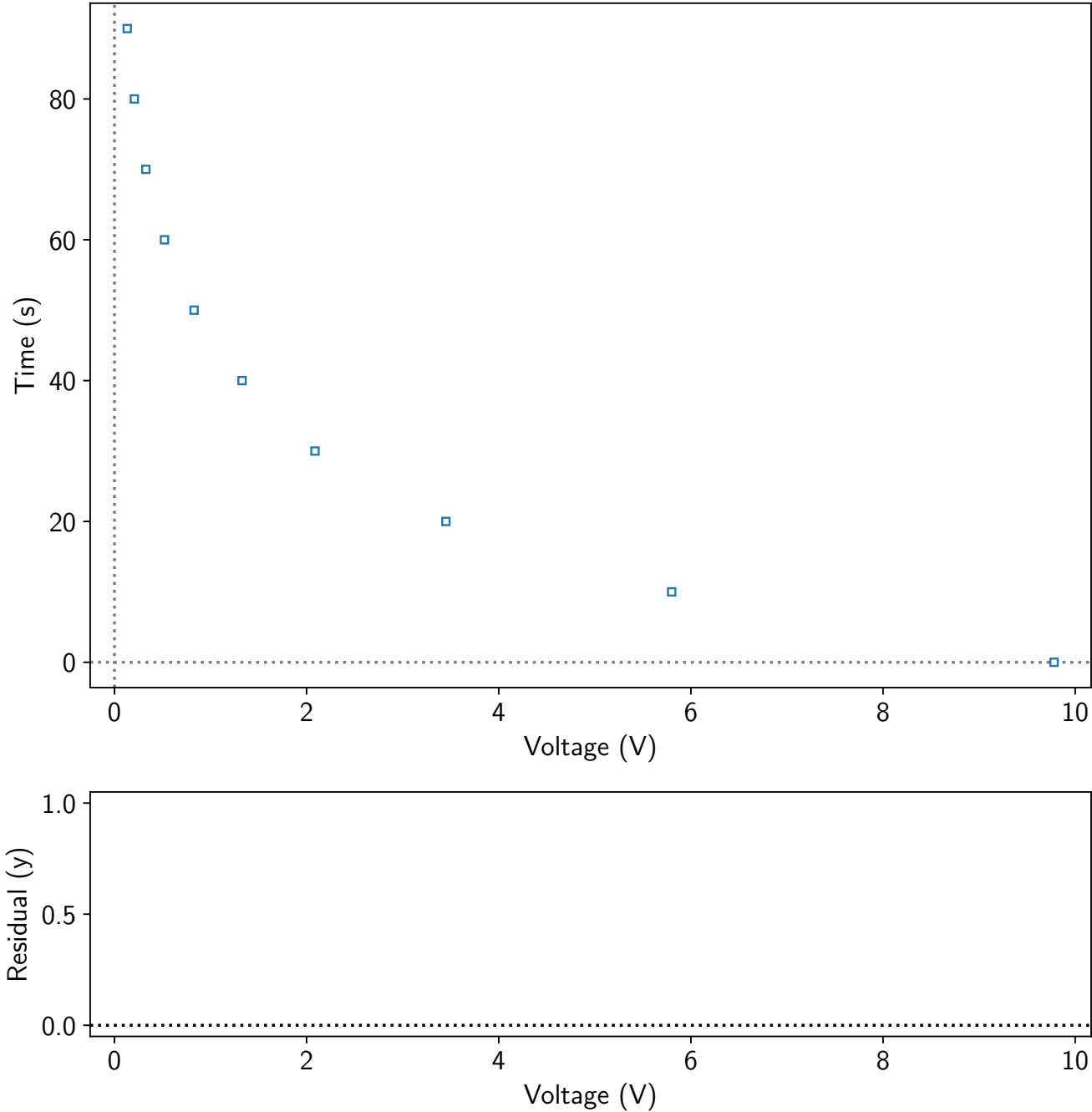
Voltage over time of a 1.8UF cpacitor
