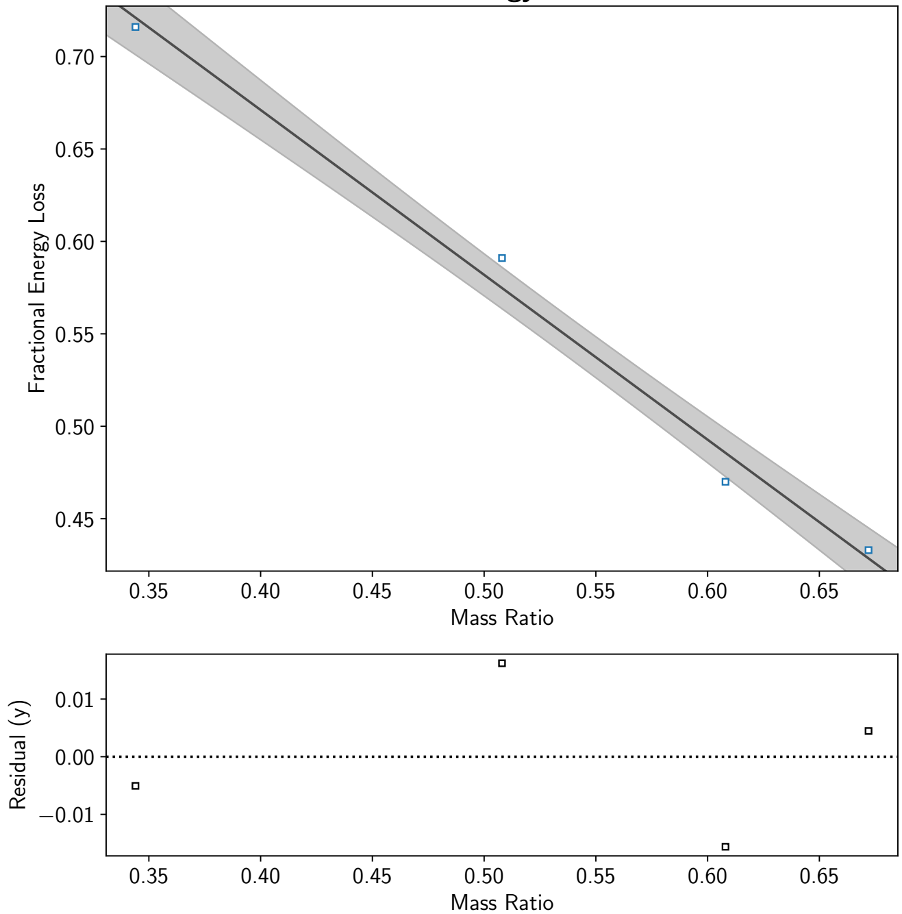
Fractional Kinetic Energy Loss vs Mass Ratio
