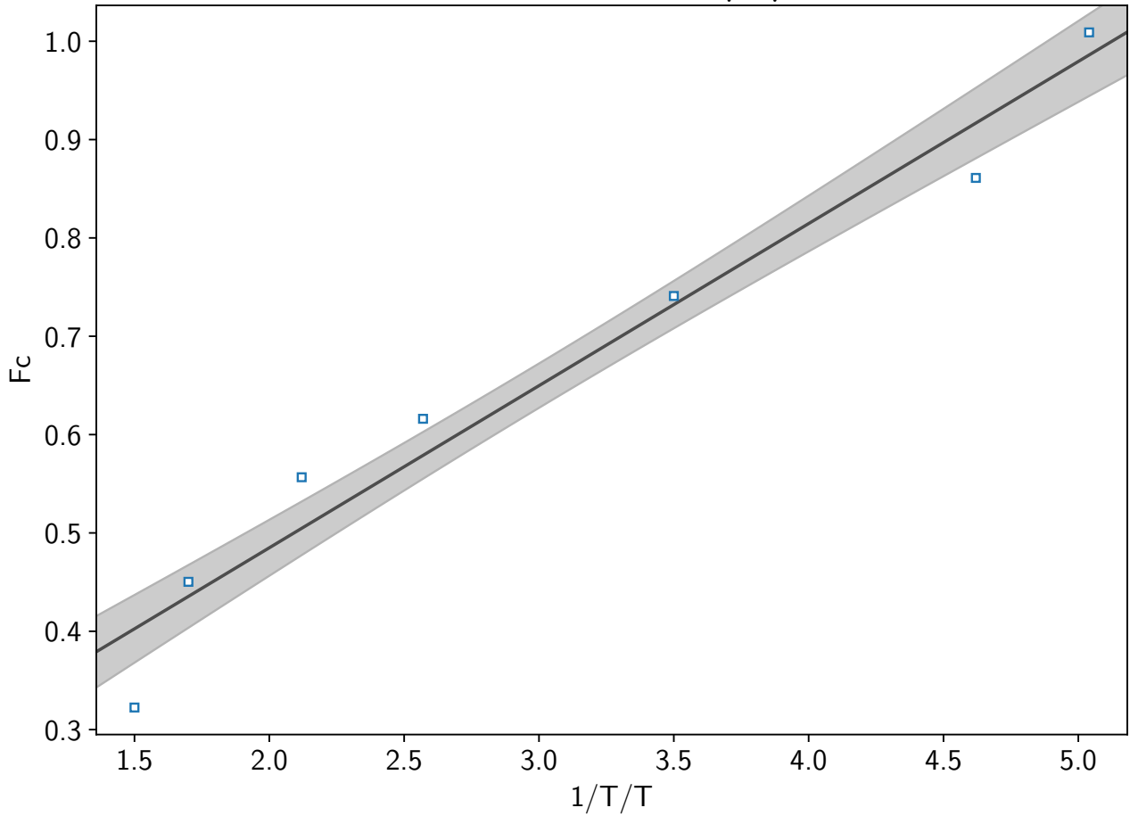
The relationship between 1/T/T and F_c
