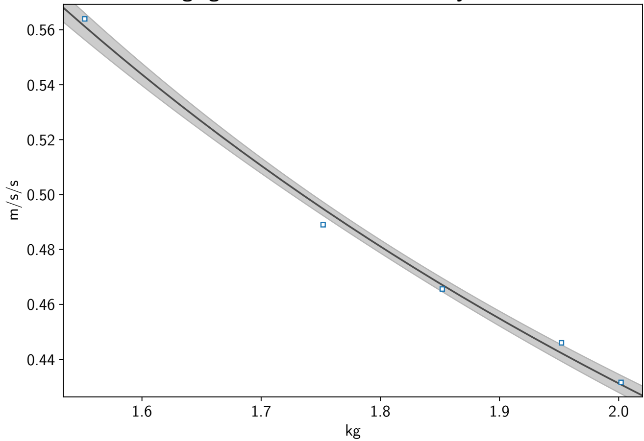
Hanging mass constant, different system mass
