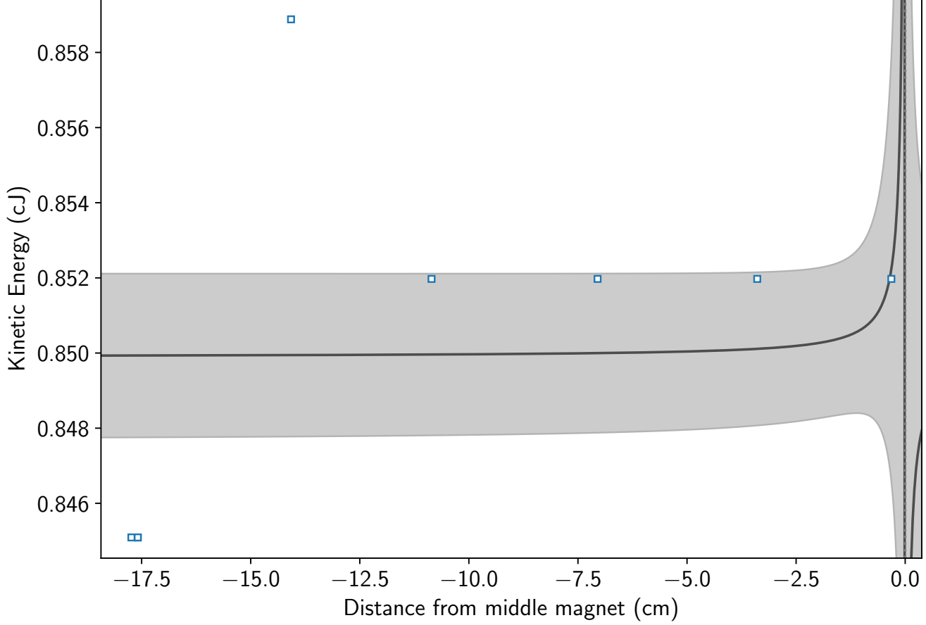
Magnet Trial 1 (mass B)
