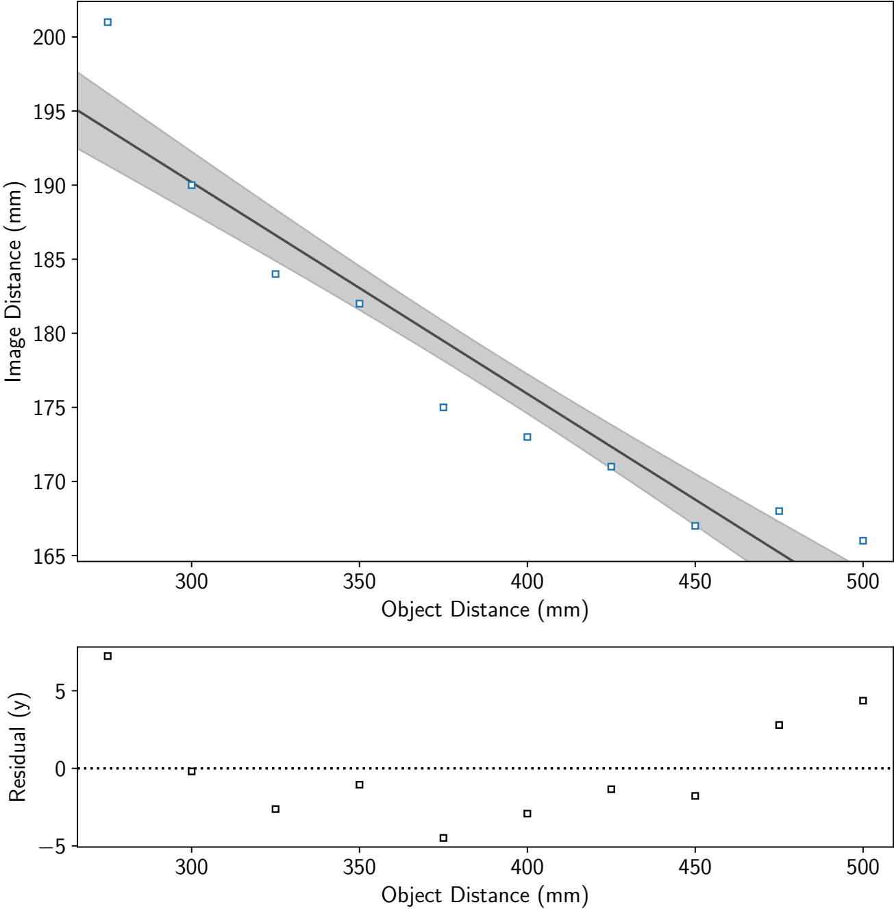
Image Distance (mm) vs. Object Distance (mm)
