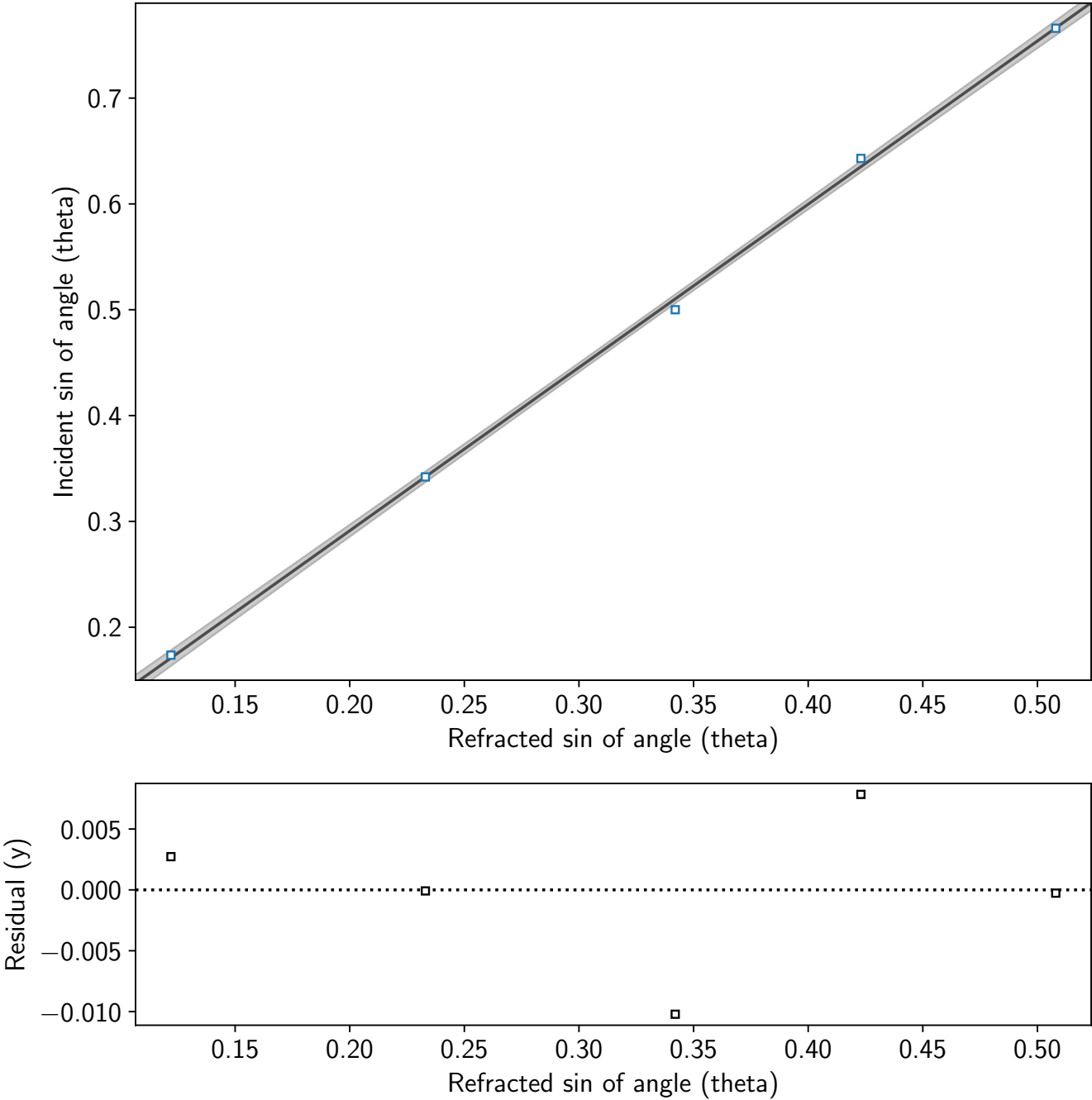
Refracted vs Incident for Light Passing Through Acrylic
