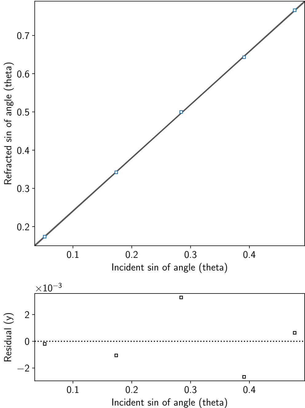
Refracted sin of Angle vs Incident sin of Angle for Light Passing Through Acrylic
