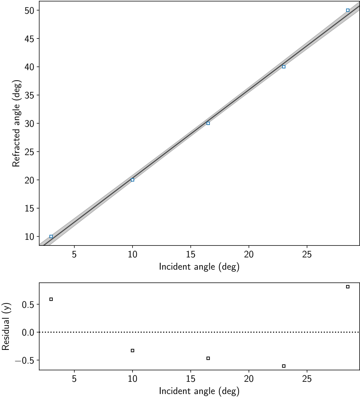
Refracted Angle vs Incident Angle for Light Passing Through Acrylic
