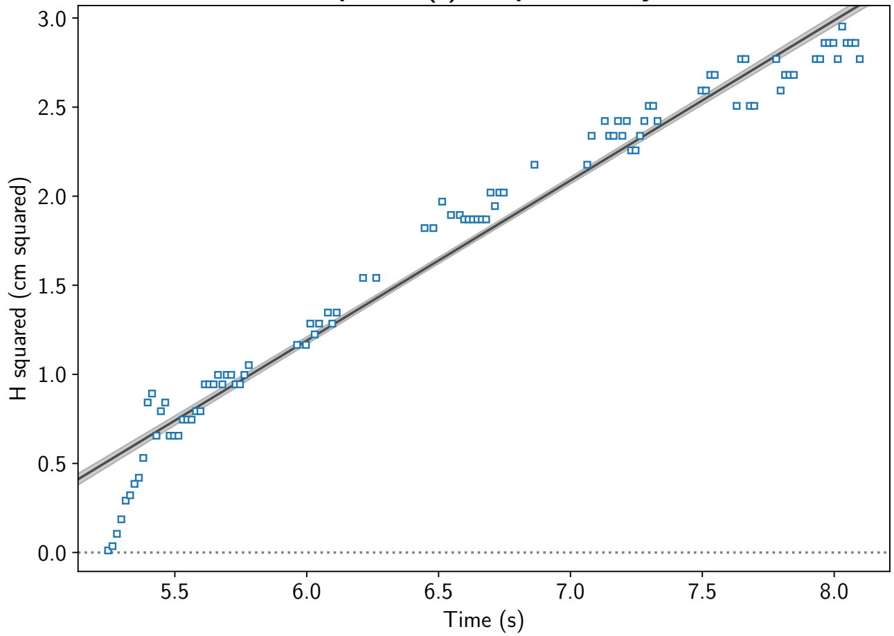
H squared (t) - 0 percent try 1
